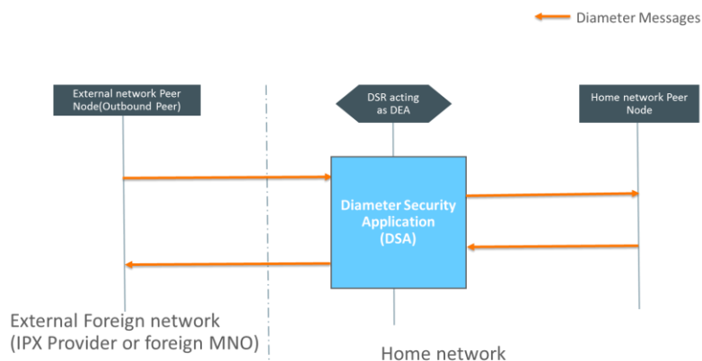
Figure 63 – Diameter Security Application (DSA)
