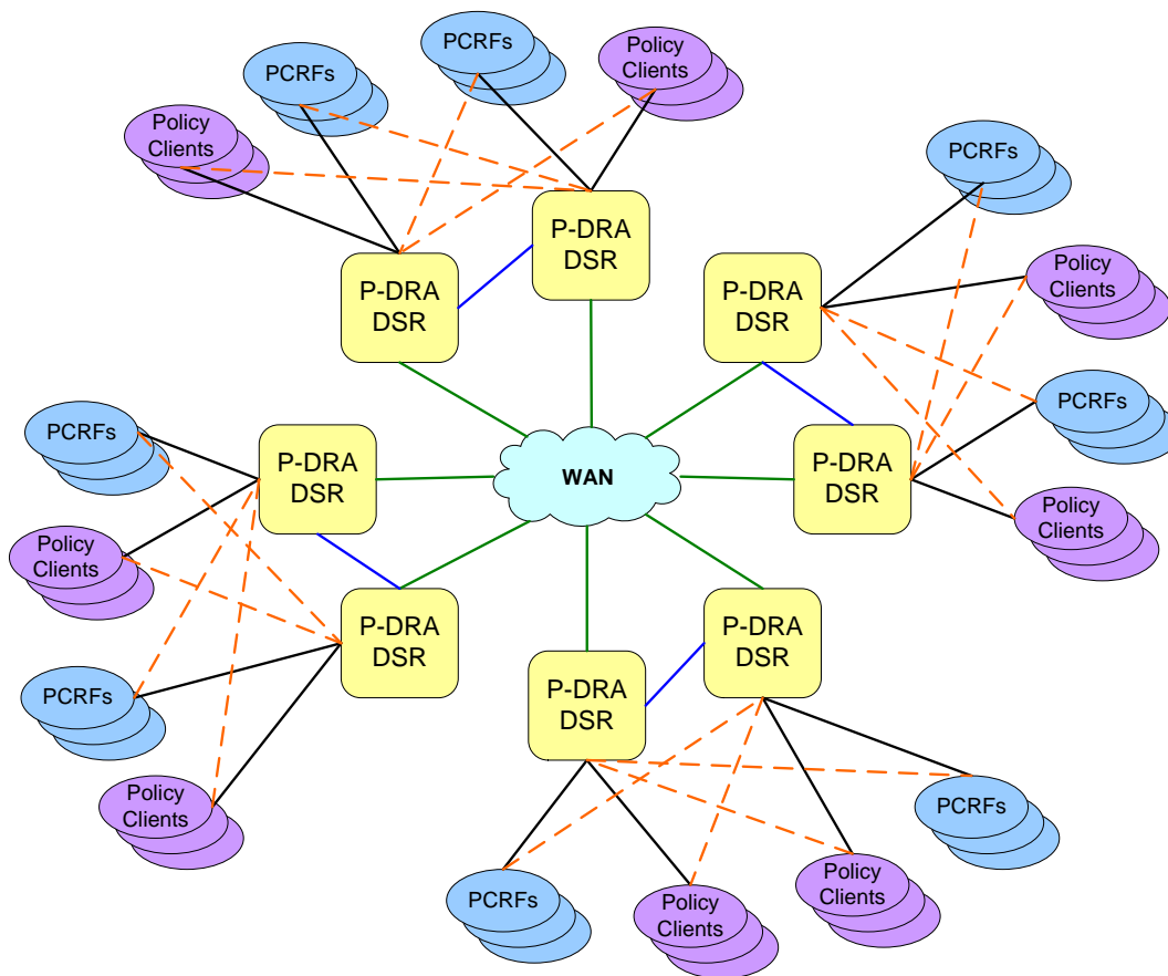
Figure 56 – Network View of P-DRA Mated Pairs
