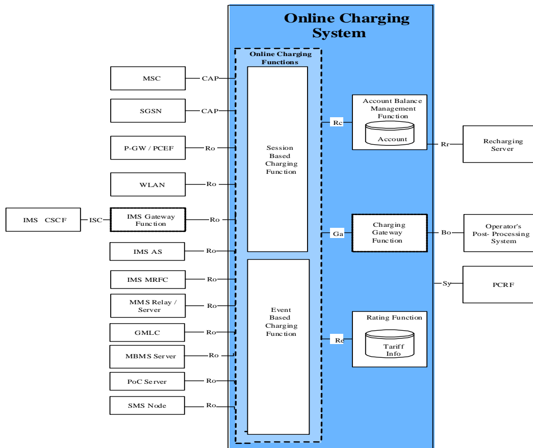
Figure 54 - Online Charging System and Architecture
