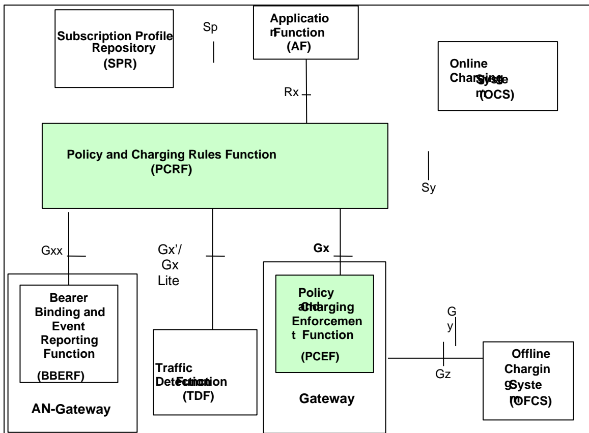
Figure 57 - Overall PCC logical architecture (non-roaming)
