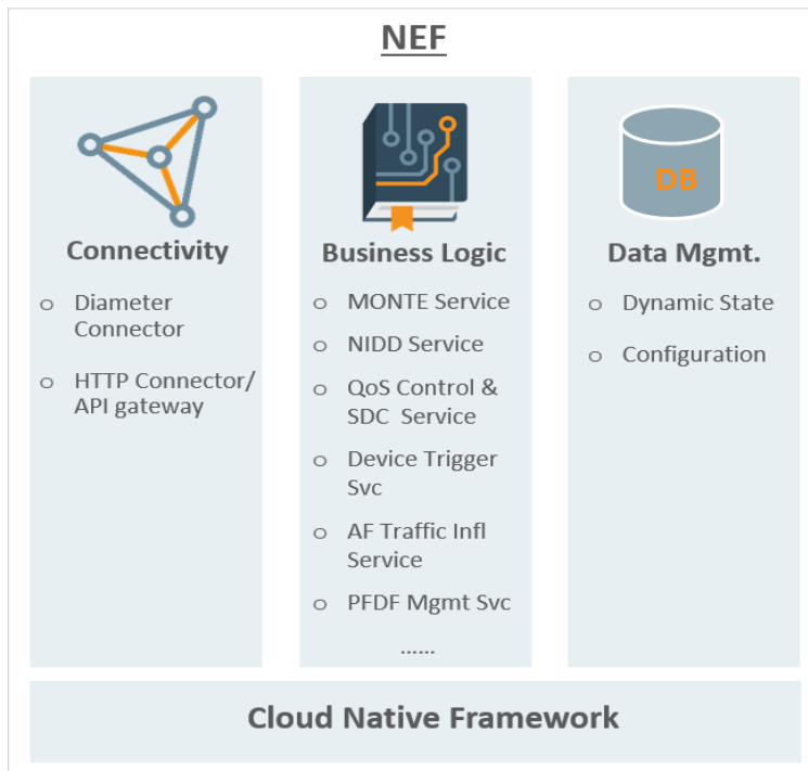
Figure 1. Oracle Communications NEF System Architecture
