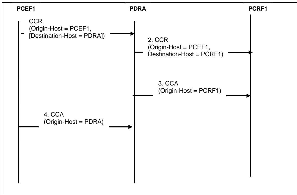
Figure 58 - PCRf topology hiding
