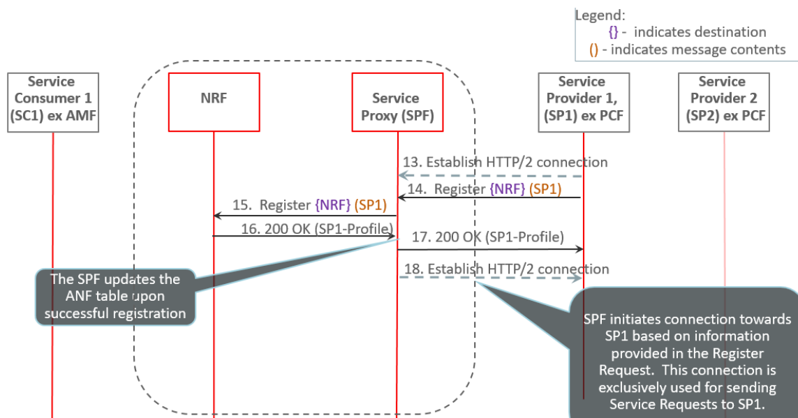
Figure 79 – NF registration call flow - Provider
