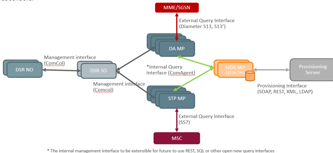
Figure 75 – EIR solution architecture.
