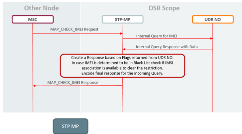
Figure 76 – SS7 EIR call flow
