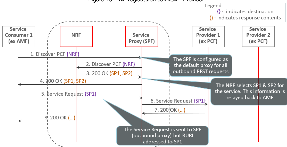
Figure 79 – NF registration call flow - Provider
