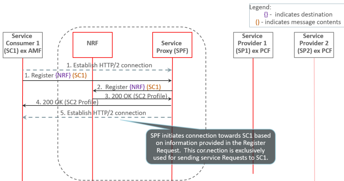
Figure 78 – NF registration call flow - Consumer
