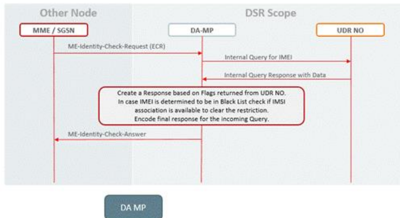
Figure 77 – S13 EIR Call Flow
